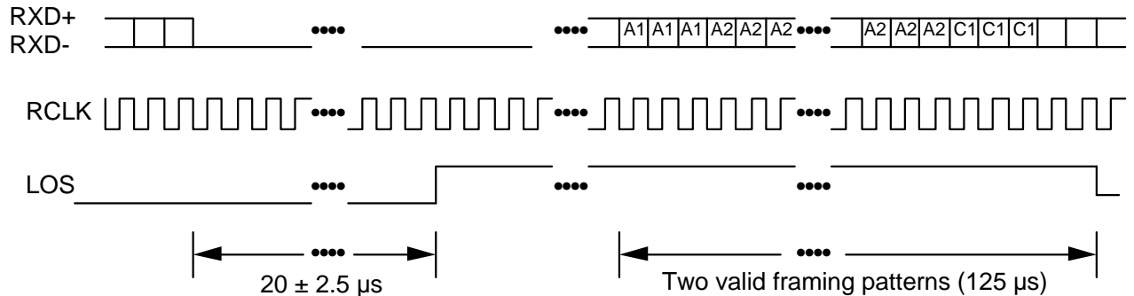
Figure 19 - Loss of Signal Declaration/Removal
